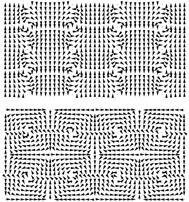
Fig. 2. The distortion field for s = 0 (top panel) and s = 1/2 (bottom panel) for geometry in Fig. 1. The vector components are (A_{xz}, A_{yz}) .
