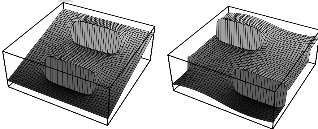
Fig. 6. The displacement fields for a screw dipole in an isotropic medium and with the geometry of Fig. 1. Two values of cell offset are shown: s = 0 (left panel) and s = 1/2 (right panel).
